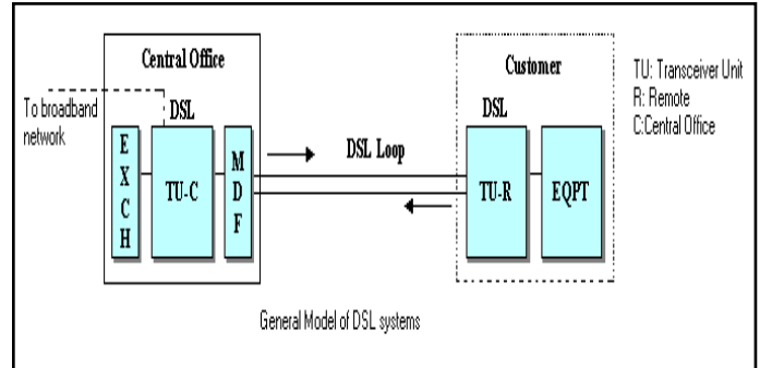
Fig. 2 : General Model of DSL systems
